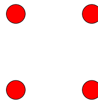
Figure 4: An edgeless graphs needs only one crayon.
