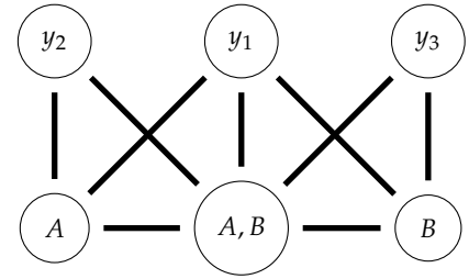
Figure 11: The final contradiction when \Delta = 3 .
